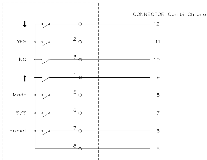
CONTROL UNIT
