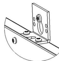
Mounting angle
